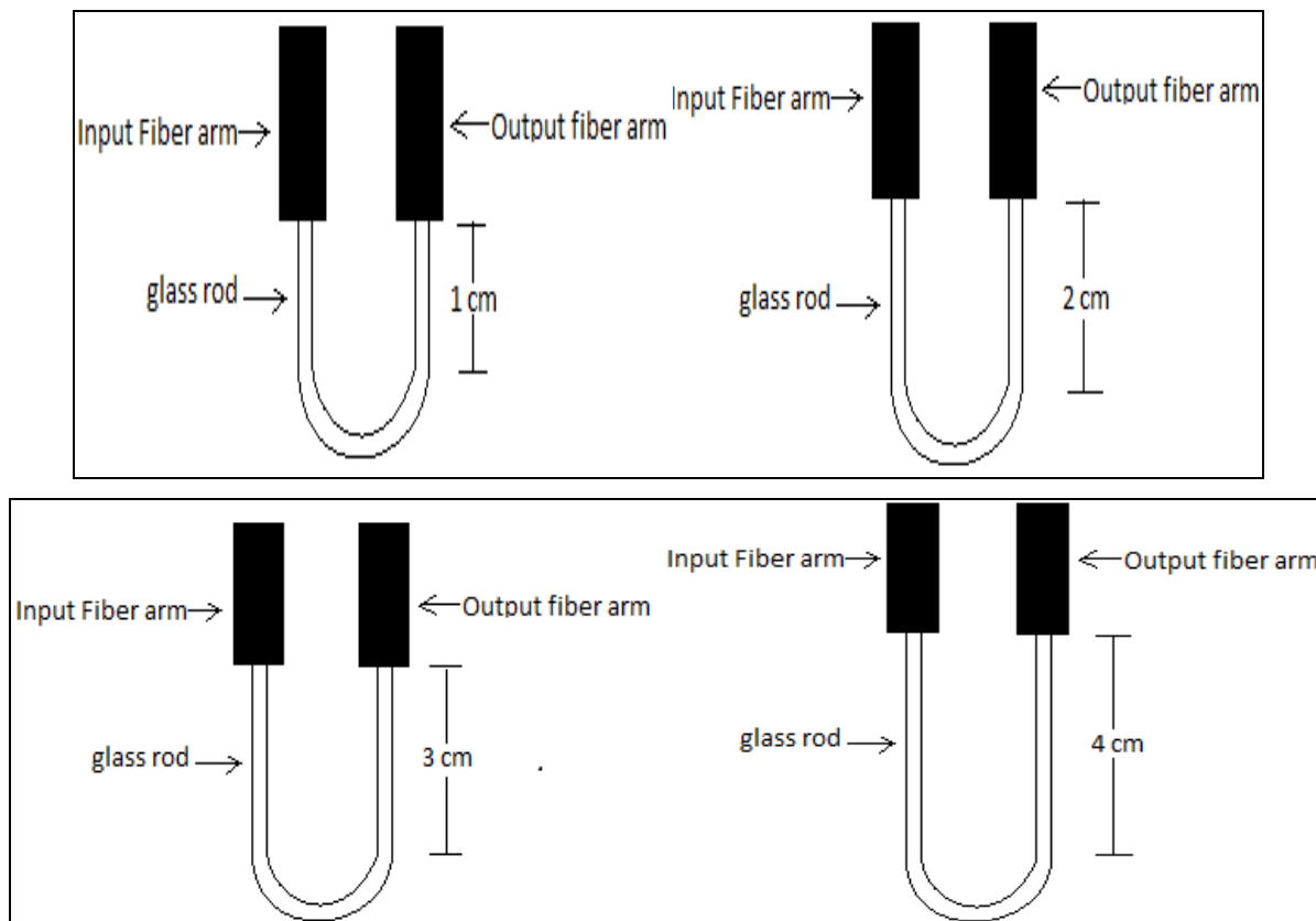
Fig. 2: U- shaped glass rods of different prong height
