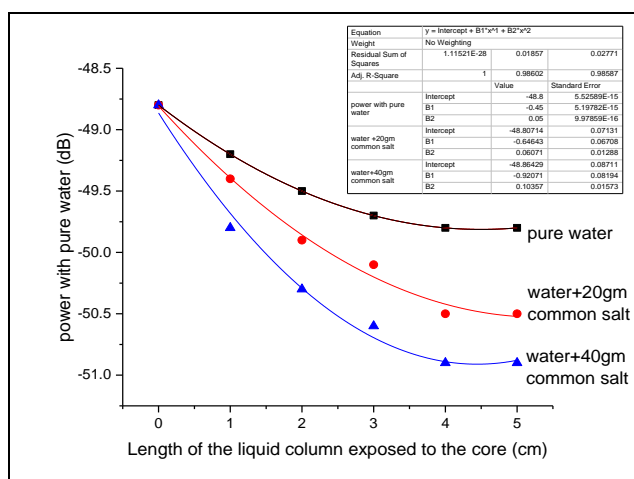
Fig. 3: Variation of power at 820nm
