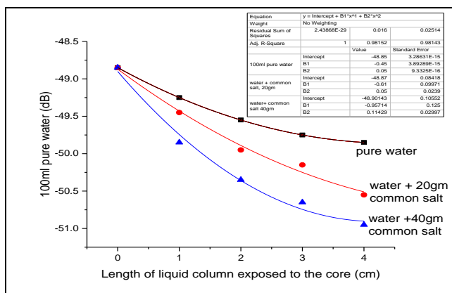
Fig. 4: Variation of power at 850nm
