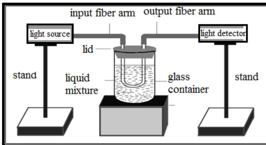
Fig. 1: Experimental arrangement
