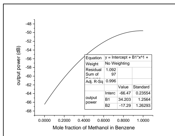
Fig. 5: Mole Fraction of CH 3 OH in C 6 H 6
