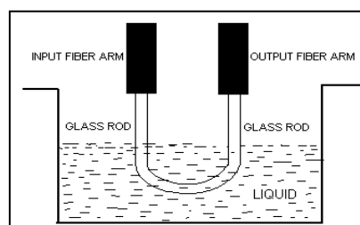
Fig. 1: Schematic of the sensor
