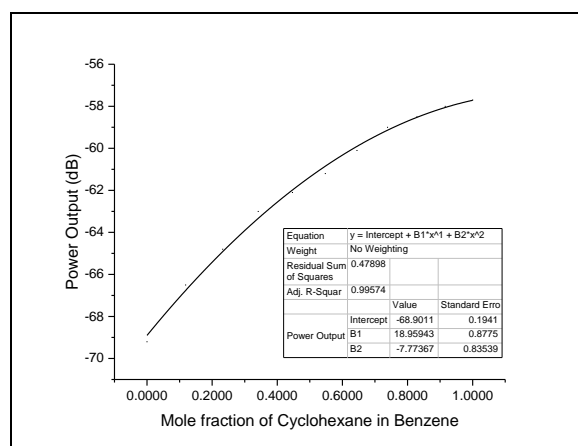
Fig. 6: Mole fraction of C 6 H 12 in C 6 H 6
