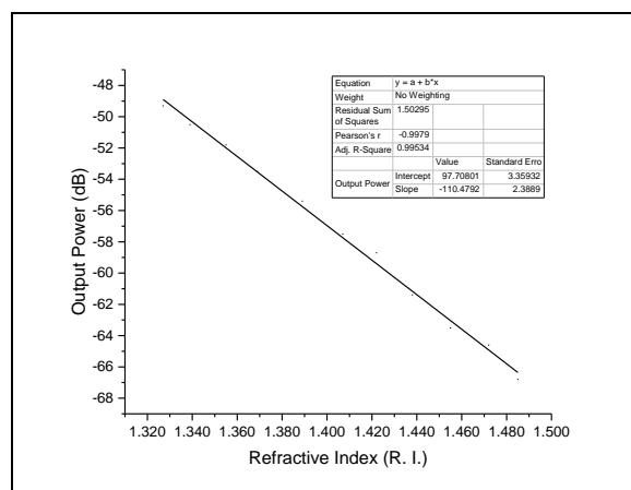
Fig.3: Methanol mixed in Benzene
