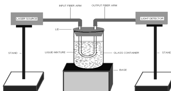
Fig. 2: Experimental arrangement of sensor
