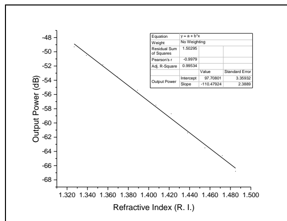
Fig.4: Cyclohexane mixed in Benzene
