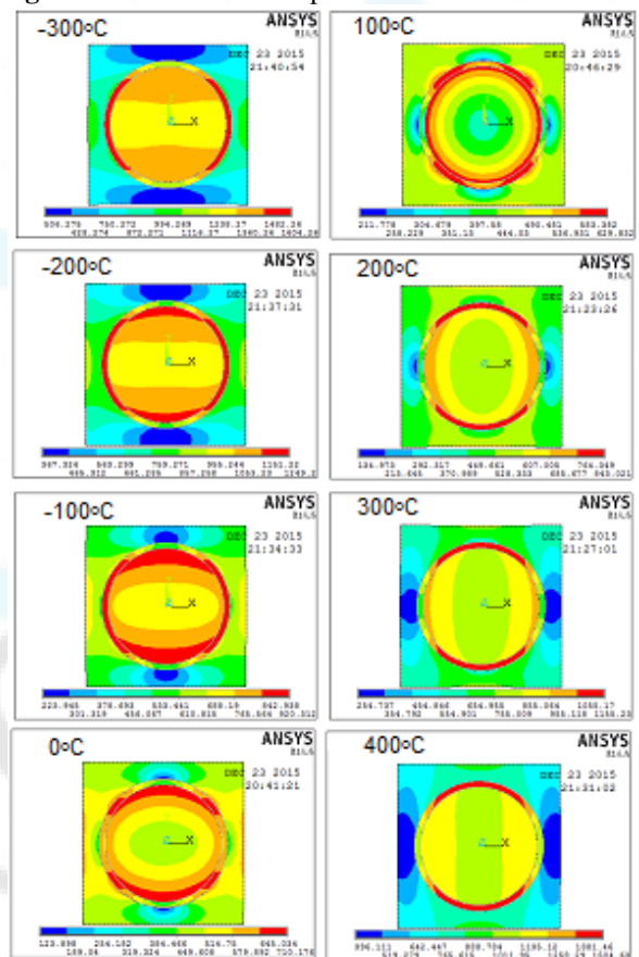
Figure 9: Raster images von Mises stress of AA7020/20% TiC composites.
