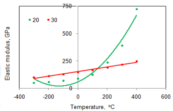
Figure 7: Influence of temperature on elastic modulus.
