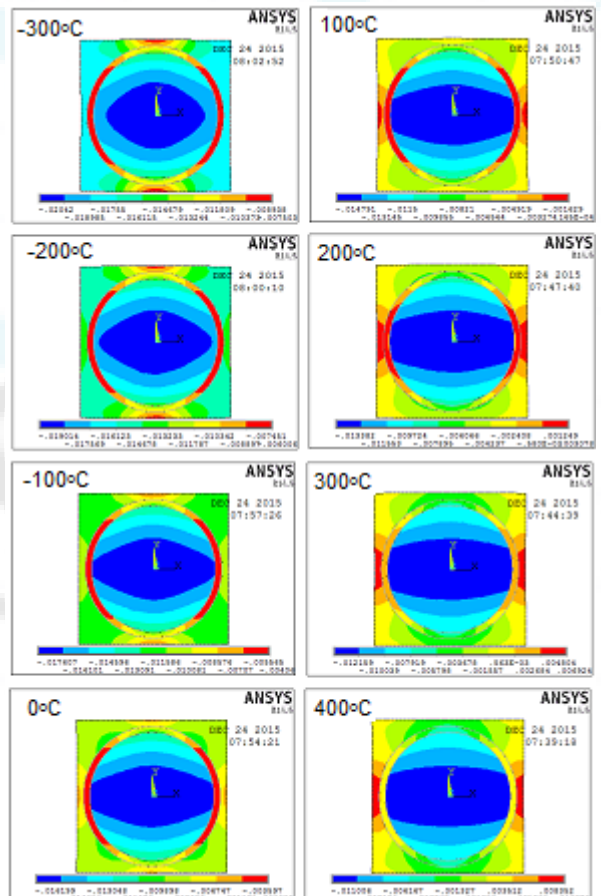
Figure 5: Raster images of thermo-elastic strain of AA7020/20% TiC composites.
