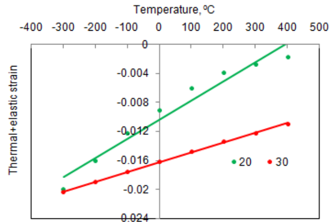
Figure 3: Influence of temperature on thermo-elastic strain.
