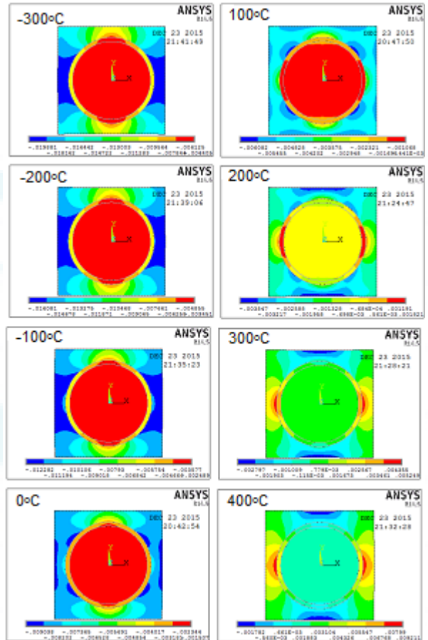
Figure 4: Raster images of thermo-elastic strain of AA7020/20% TiC composites.
