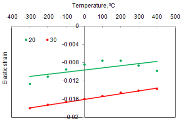
Figure 2: Influence of temperature on elastic strain.
