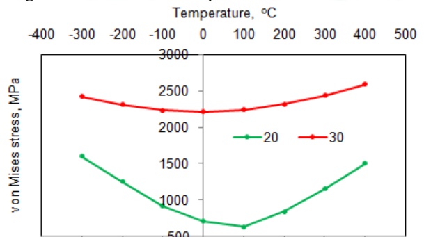
Figure 8: Influence of temperature on von Mises stress.
