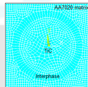
Figure 1: The RVE model
