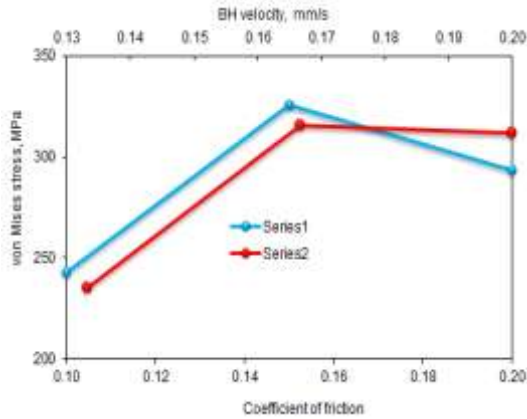
Fig. 6: The von Mises stress as a function of COF and BH velocity.
