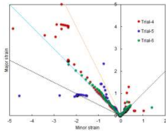
Fig. 13: Forming limit diagram with damage in the cups drawn at temperature 400°C.
