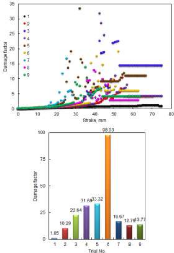
Fig. 15: Damage factors under different trials.
