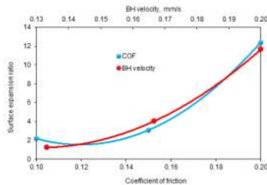
Fig. 10: The surface expansion ratio as a function of COF and BH velocity.
