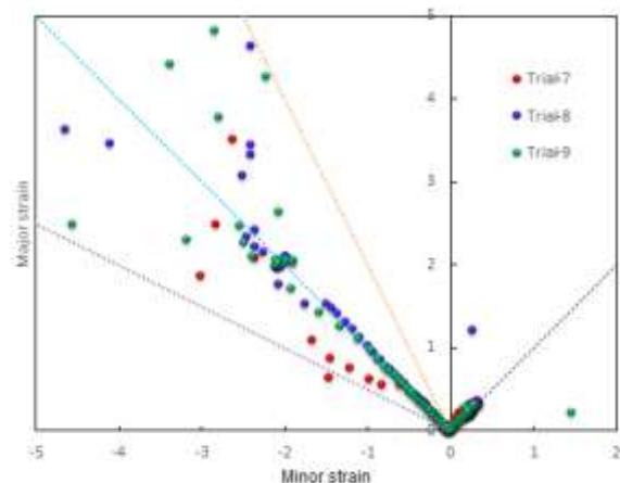
Fig. 14: Forming limit diagram with damage in the cups drawn at temperature 500°C.
