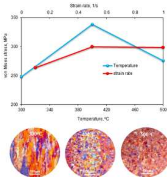
Fig. 3: The von Mises stress as a function of temperature and strain rate.
