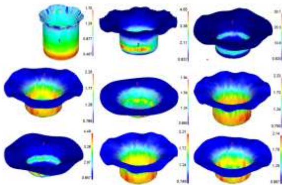
Fig. 11: Effect of process parameters on the surface expansion ratio.
