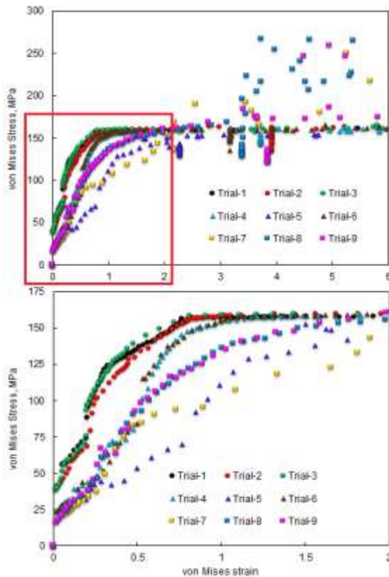
Fig. 7: Effect of von Mises strain on the von Mises stress.
