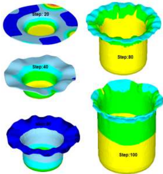
Fig. 2: Formation of cylindrical cup at different steps of FEA simulation.
