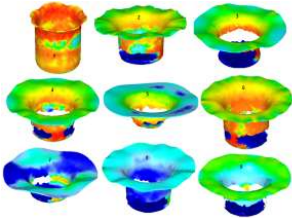
Fig. 16: Damages of the cups drawn under different trials.
