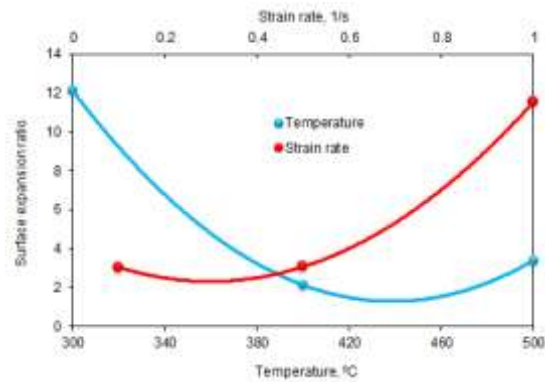
Fig. 9: The surface expansion ratio as a function of temperature and strain rate.
