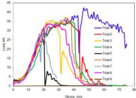
Fig. 8: Applied load as a function punch stroke.
