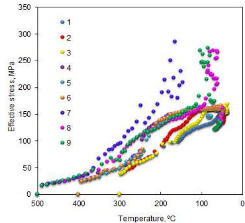
Fig. 4: Effect of temperature on von Mises stress for all trials.
