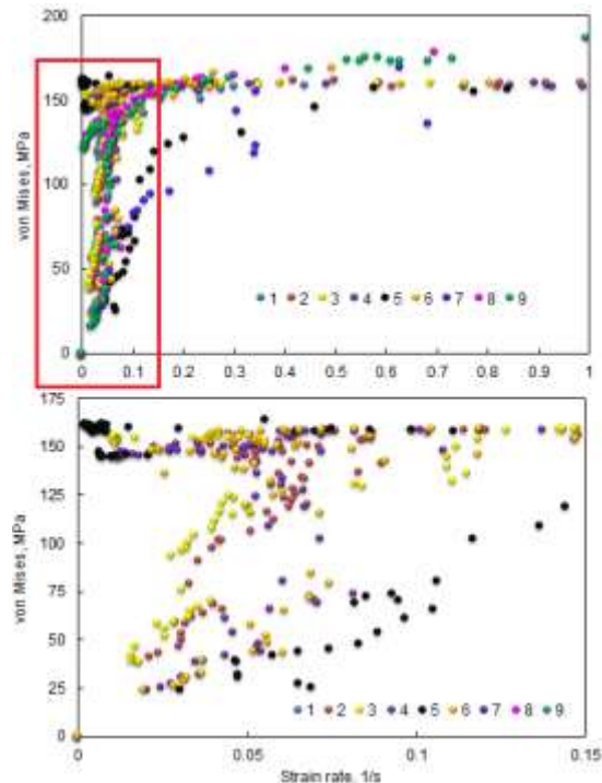
Fig. 5: Effect of strain rate on von Mises stress for all trials.
