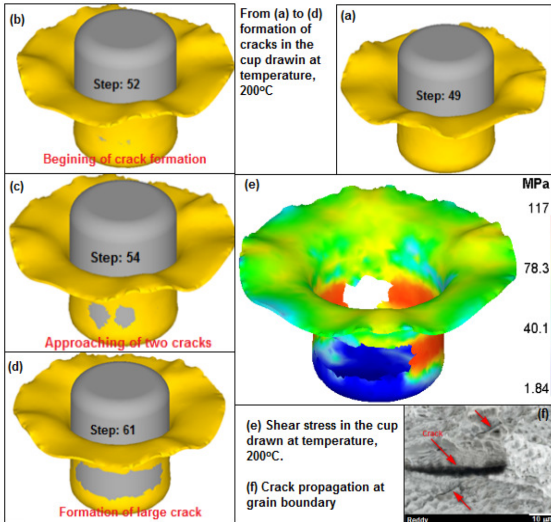
Figure 8 Important features of the cup drawn at temperature 200°C
