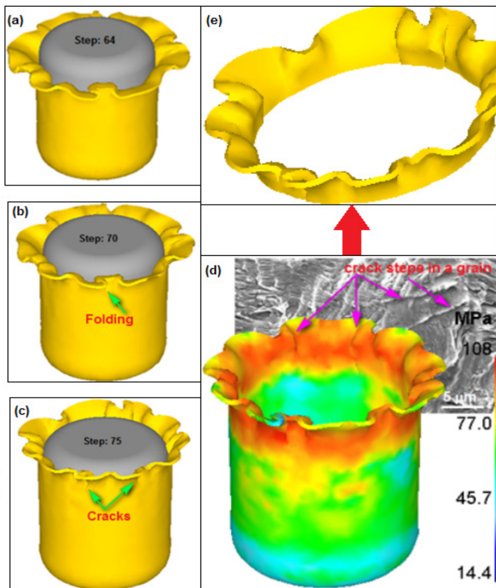
Figure 9 Formation of folds and cracks in the cup drawn at temperature 275°C
