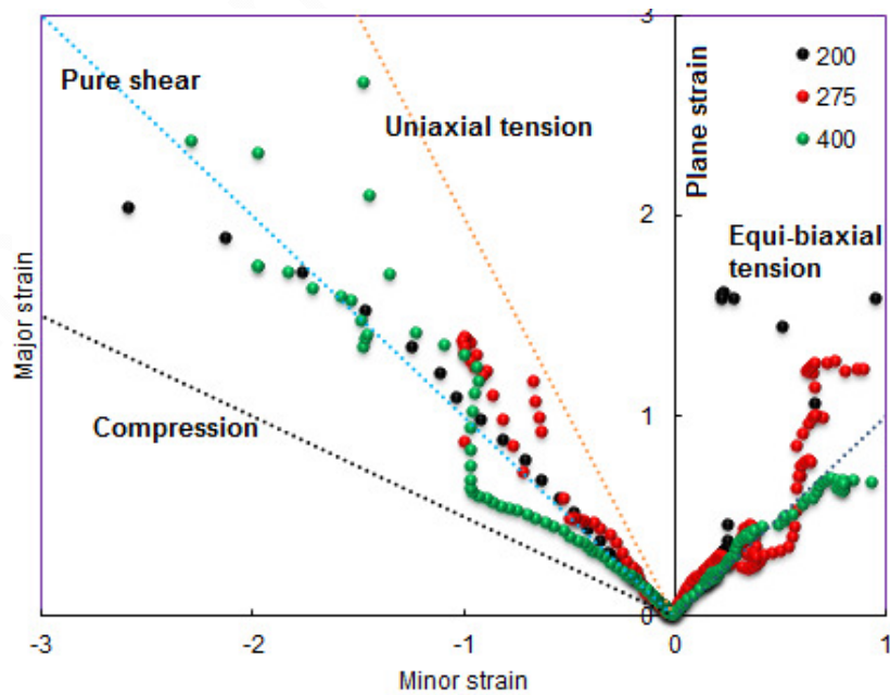
Figure 5 Forming limit diagram of the cups drawn at different temperatures
