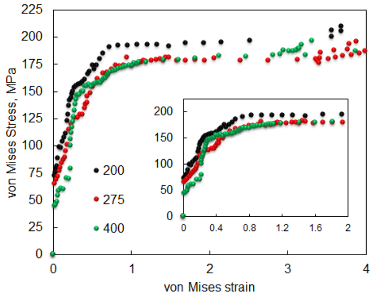
Figure 4 The von Mises stress as a function of temperature (the other parameters are maintained at constant levels).
