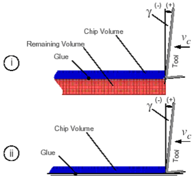
Fig-4 Model based on the contact detachment technique
