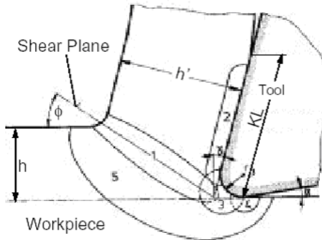
Fig-2. Section through the cutting area and resultant chip, showing the deformation zones [2]
