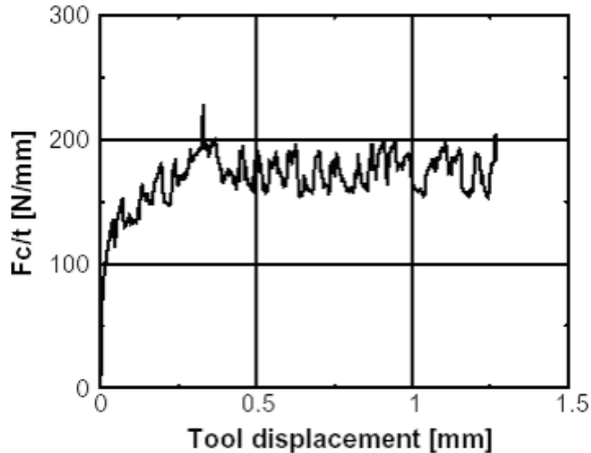
Fig-6. Tool displacement vs. cutting force at a cutting speed of 4000m/min (0,18% carbon steel)
