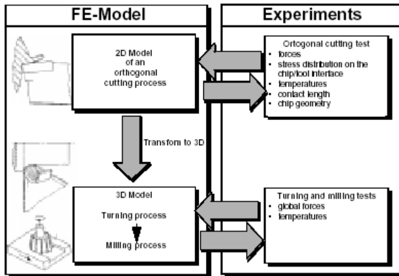
Fig.1 shows schematically the different zones, which have an important influence within chip formation.
