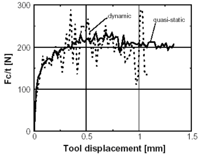
Fig-8. Cutting forces of quasi static analysis in comparison with a dynamic simulation
