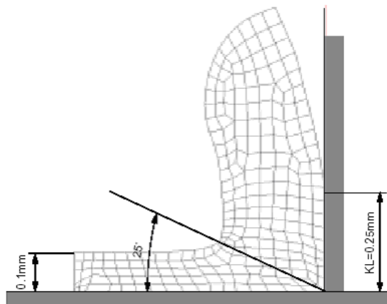
Fig-5. Calculated chip geometry at a cutting speed of 4000 m/min for a 0.18% carbon steel
