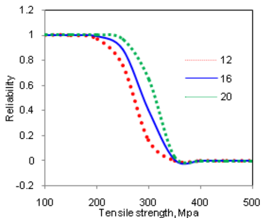
Figure 12: Reliability graphs for tensile strength of /6061/Al 2 O 3 .
