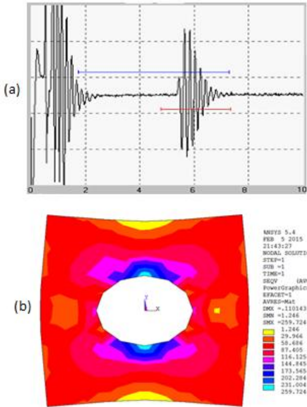
Figure 6: Porosity in 6061/Al 2 O 3 composite (particles of 10µm size and V p = 20%)
