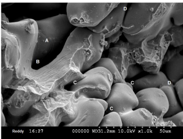
Figure 4: Cracking of Al_2O_3 particle of 30\mu m size
