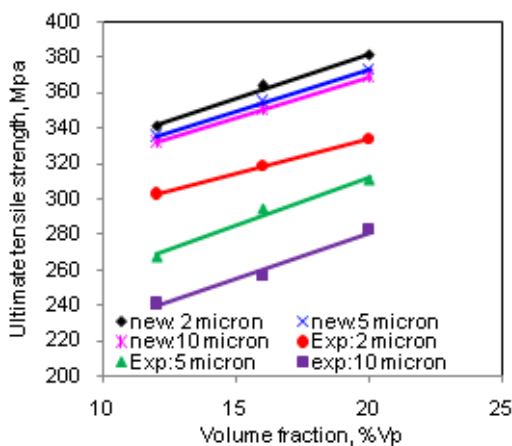
Figure 10: Comparison of proposed criterion with experimental values
