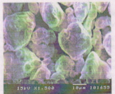
Fig. 3 SEM Photograph of Lead Powder
