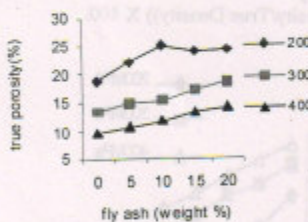
Fig. 13 Effect of Fly Ash on True Porosity
