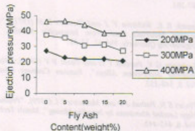
Fig. 8 Effect of Fly Ash Content on Ejection Pressure
