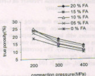
Fig. 12 Effect of Compaction Pressure on True Porosity
