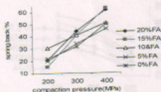
Fig. 11 Effect of Compaction Pressure on Spring Back
