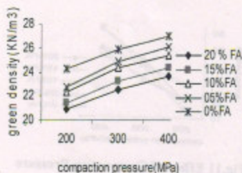
Fig. 9 Effect of Compaction Pressure on Green Density
