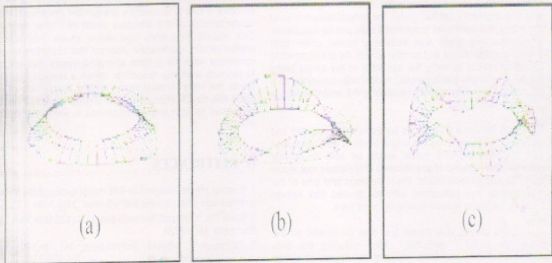
Fig 6. Effect Disk (a) Zero, (b) Two, and (c) Four Nodal Diameters
