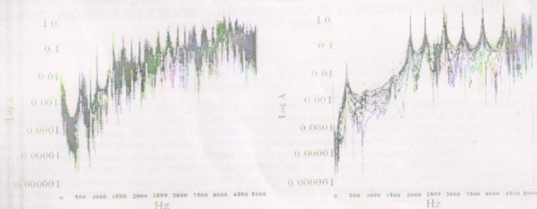
Fig 1. Frequency Response Functions from Loose and Tight Structures
