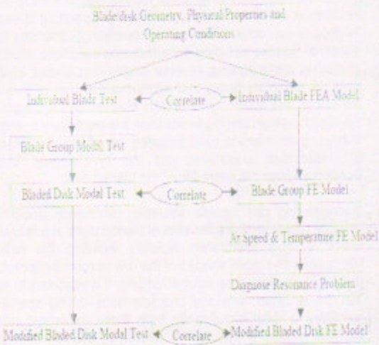
Fig 2. Flowchart of Response Investigation
