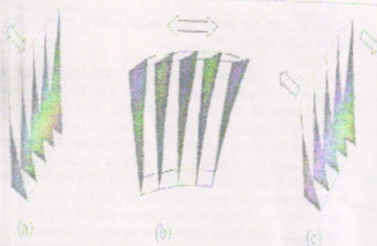
Fig 4. Fundamental Modes. (a) Axial, (b) Tangential and (c) Twist.
